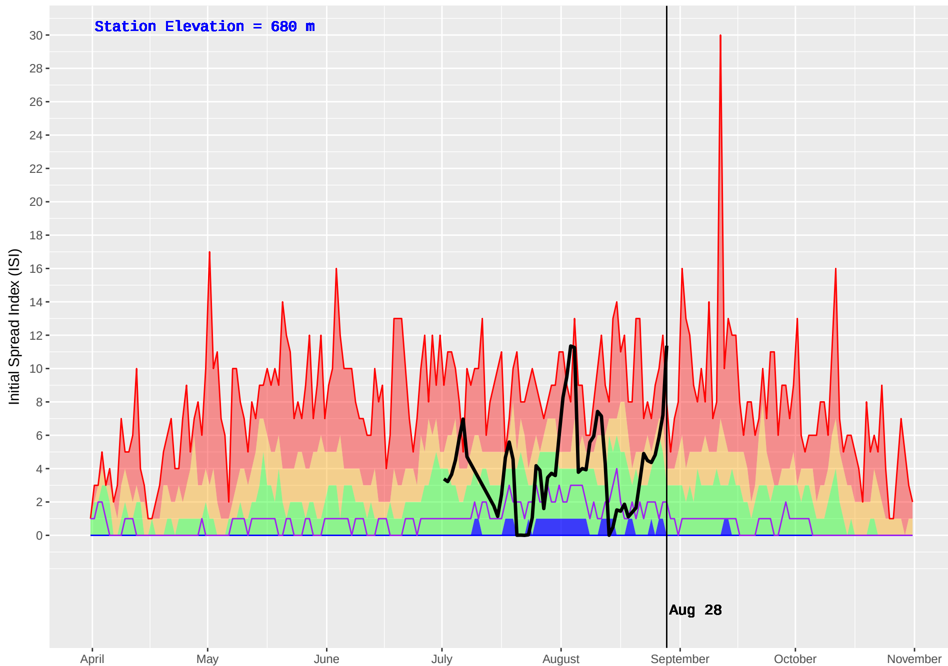
SUMMIT (11) : Historical (1985–2016) and Current (2017) Noon Initial Spread Index (ISI)
